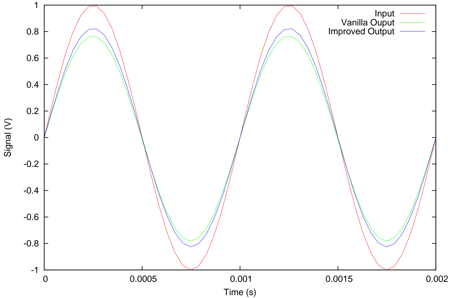
Improvement of Transient Response at 1kHz
